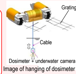
Image of hanging of dosimeter and camera
