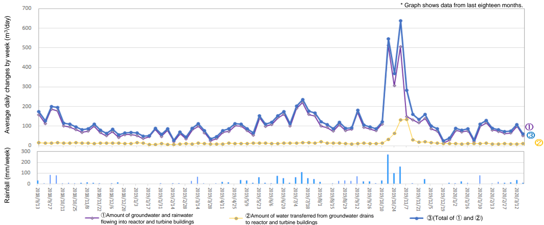
Amount of water transferred from groundwater drains to reactor and turbine buildings (From Mar 12, 2020 to Mar 18, 2020)
