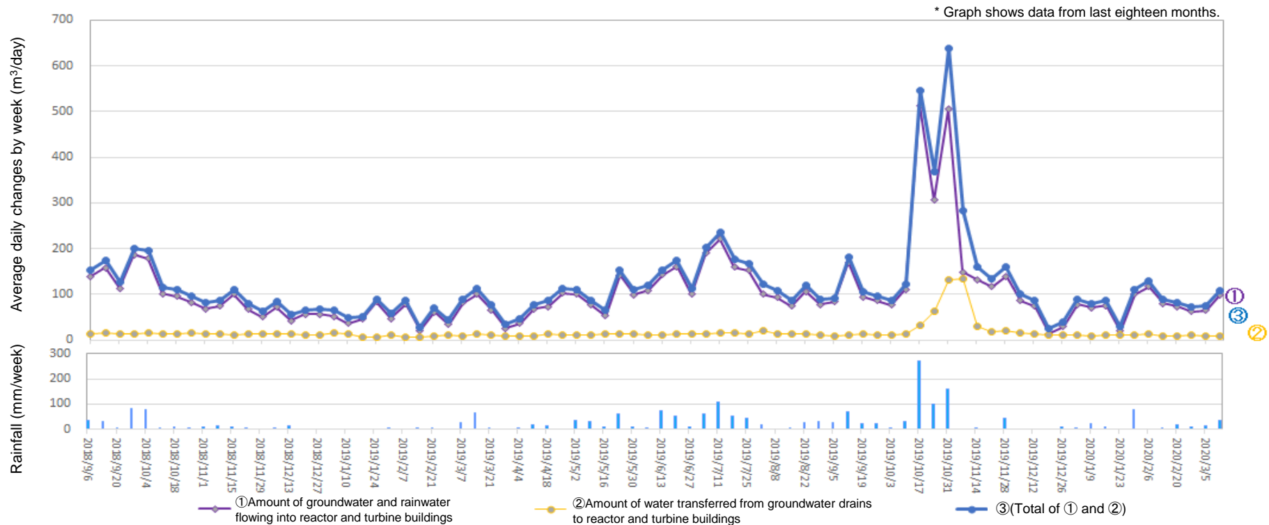
Amount of water transferred from groundwater drains to reactor and turbine buildings (From Mar 5, 2020 to Mar 11, 2020)
