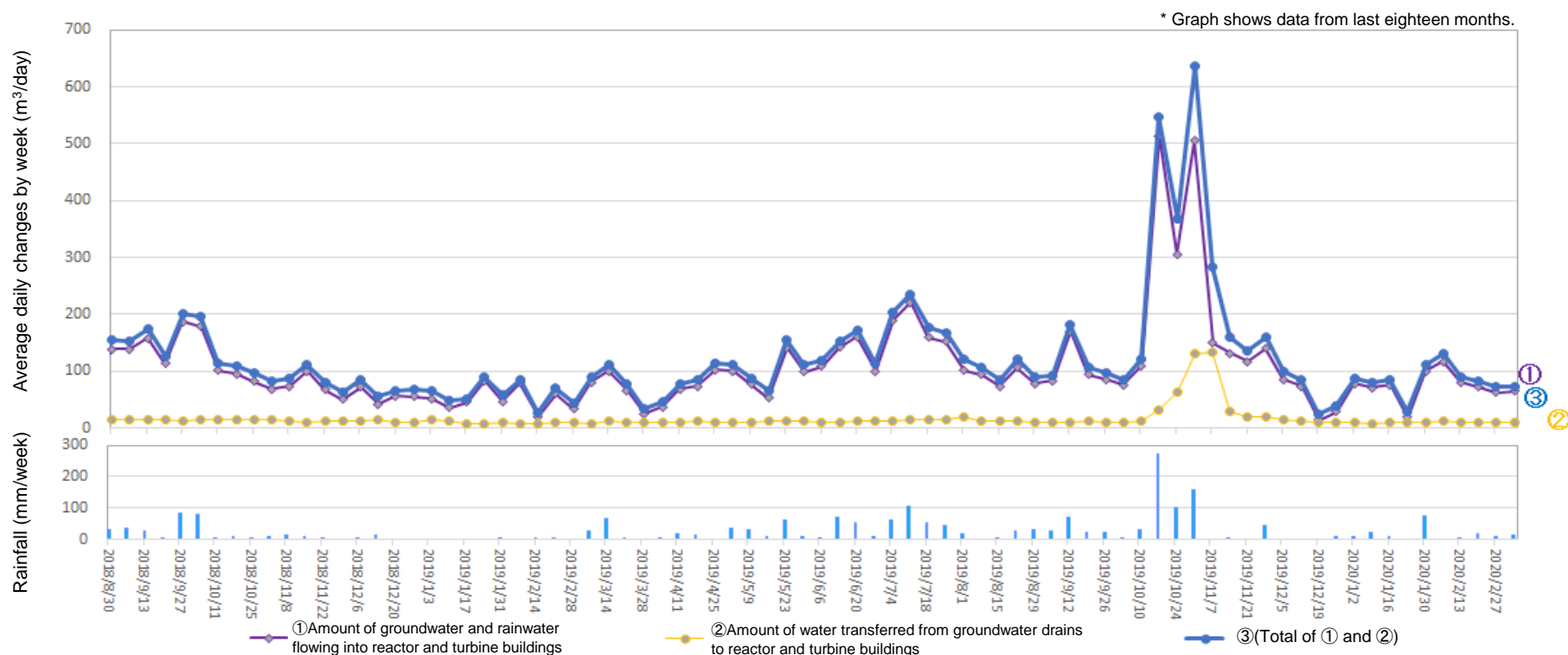
Amount of water transferred from groundwater drains to reactor and turbine buildings (From Feb 27, 2020 to Mar 4, 2020)
