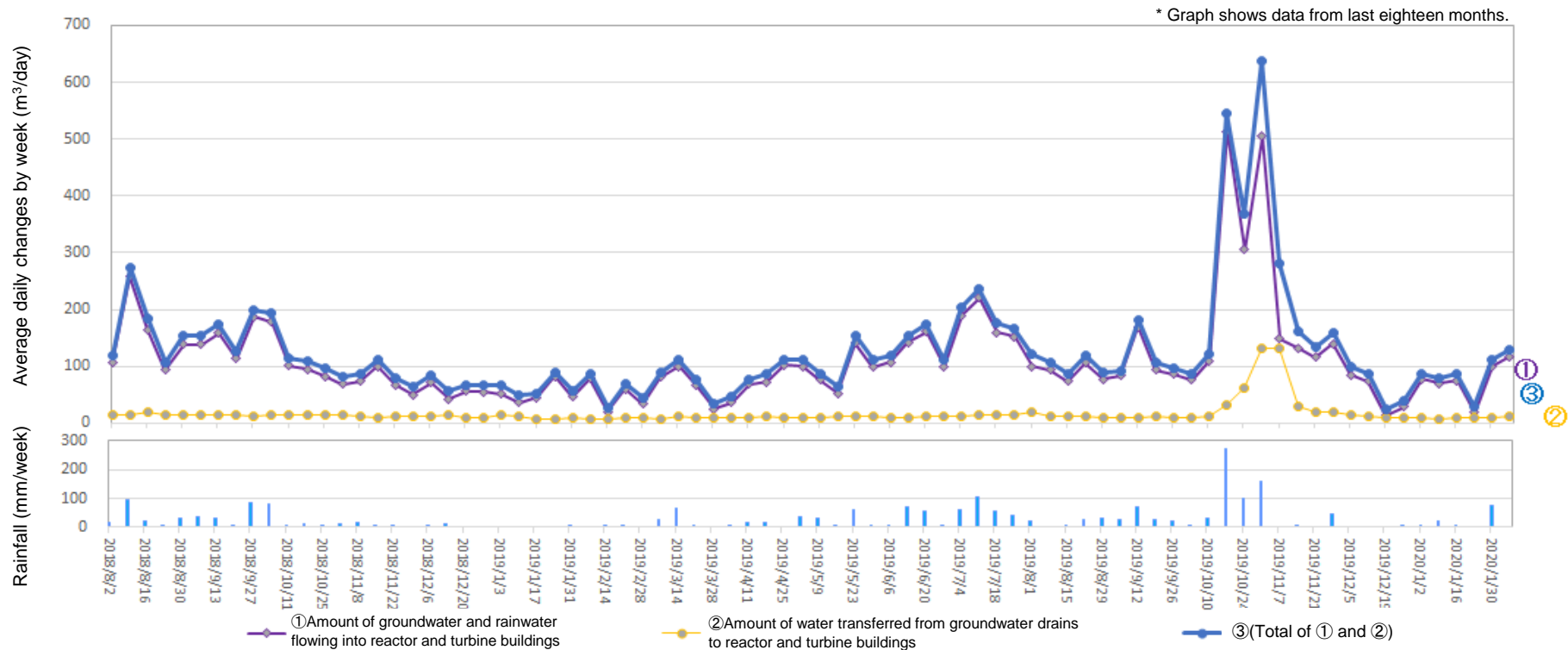
Amount of water transferred from groundwater drains to reactor and turbine buildings (From Jan 30, 2020 to Feb 5, 2020)
