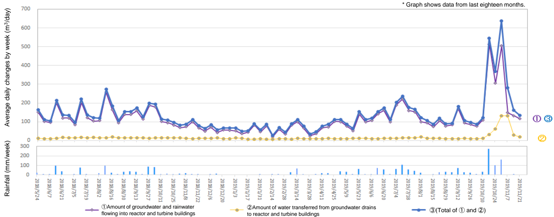
Amount of water transferred from groundwater drains to reactor and turbine buildings (From Nov 14, 2019 to Nov 20, 2019)
