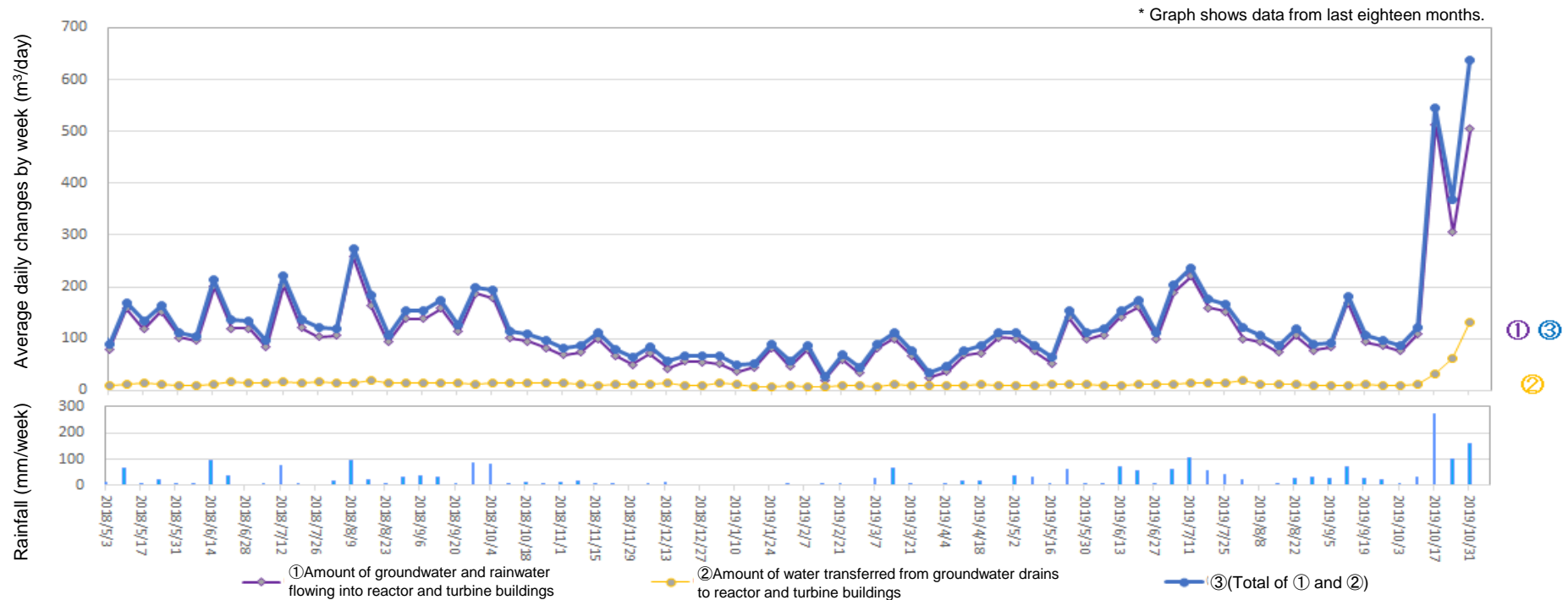
Amount of water transferred from groundwater drains to reactor and turbine buildings (From Oct 24, 2019 to Oct 30, 2019)
