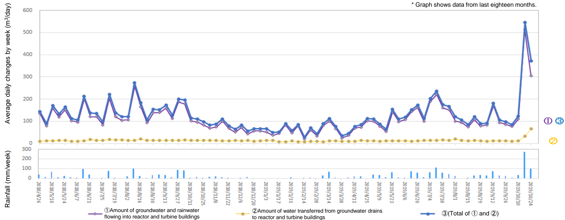
Amount of water transferred from groundwater drains to reactor and turbine buildings (From Oct 17, 2019 to Oct 23, 2019)
