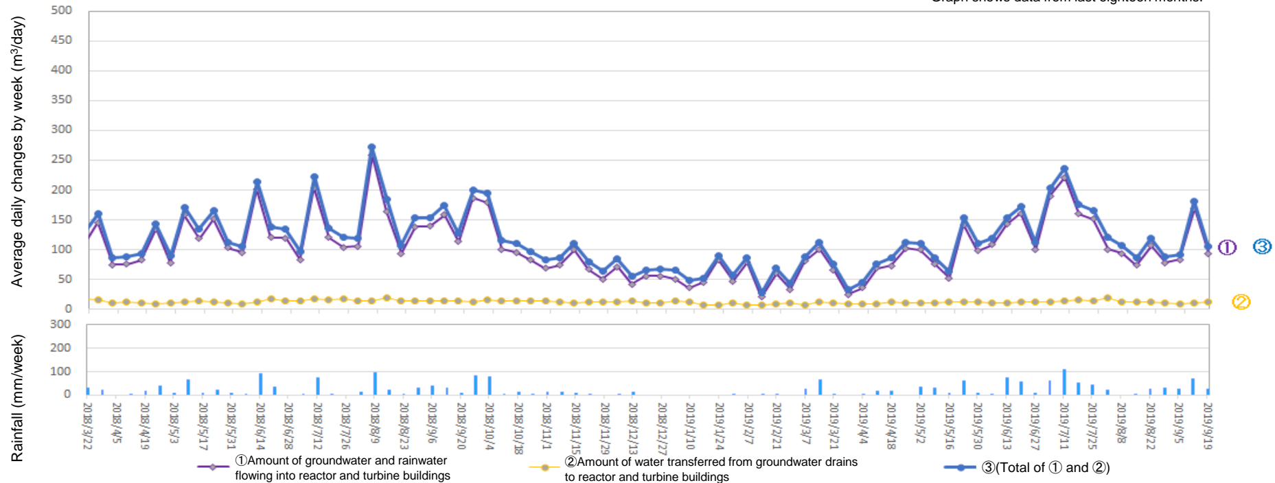
Amount of water transferred from groundwater drains to reactor and turbine buildings (From Sept 12, 2019 to Sept 18, 2019)
