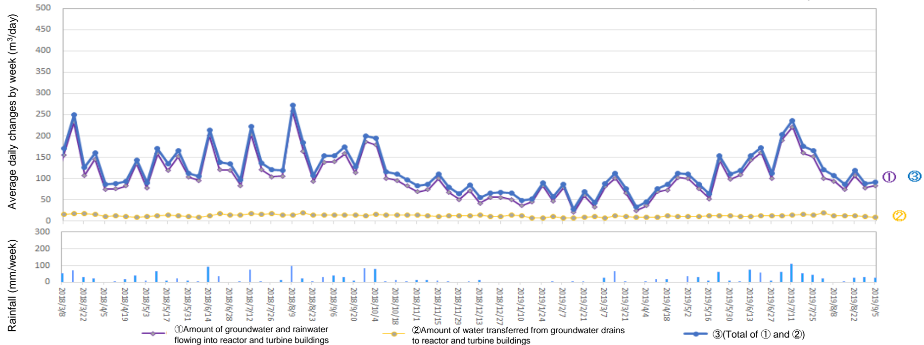
Amount of water transferred from groundwater drains to reactor and turbine buildings (From Aug 29, 2019 to Sept 4, 2019)
