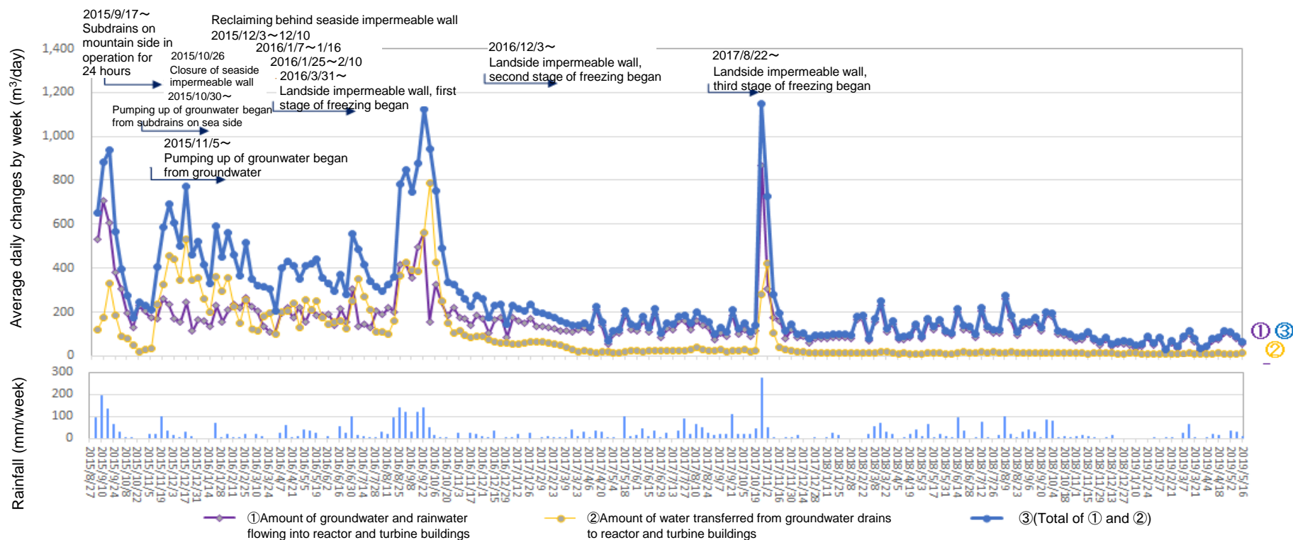
Amount of water transferred from groundwater drains to reactor and turbine buildings
