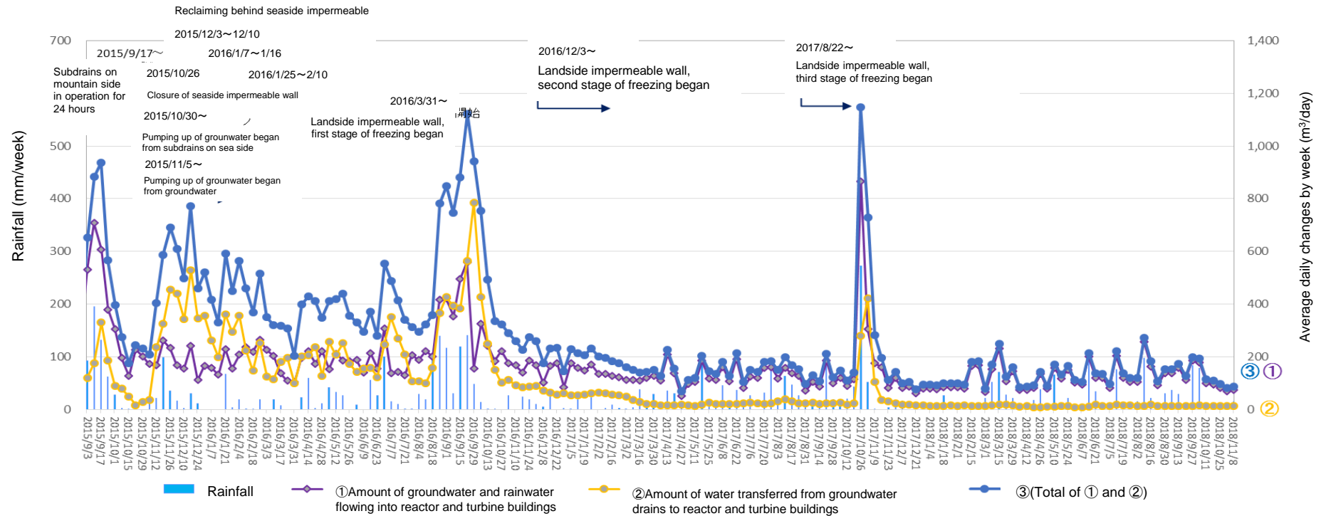
Amount of water transferred from groundwater drains to reactor and turbine buildings (From November 1, 2018 to November 7, 2018)
