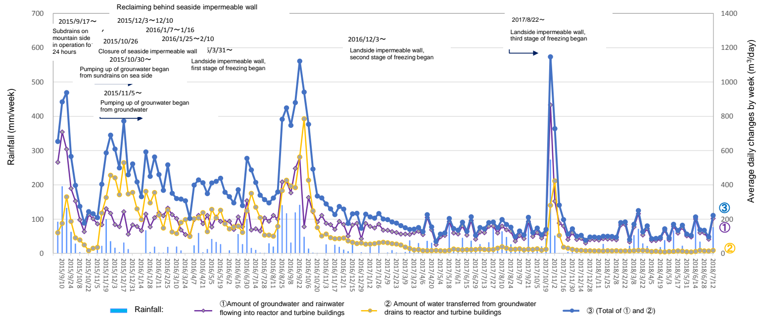
Amount of water transferred from groundwater drains to reactor and turbine buildings (From July 5, 2018 to July 11, 2018)
