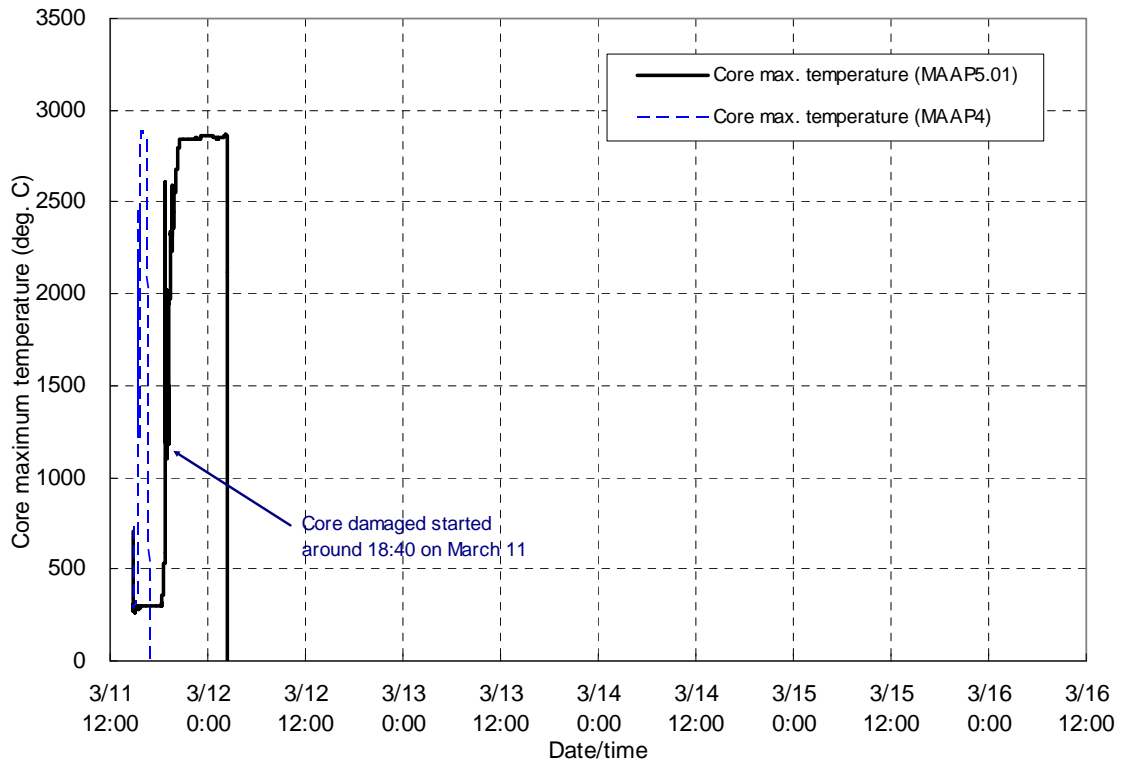
Figure 1-4 Core temperature changes of Unit-1
