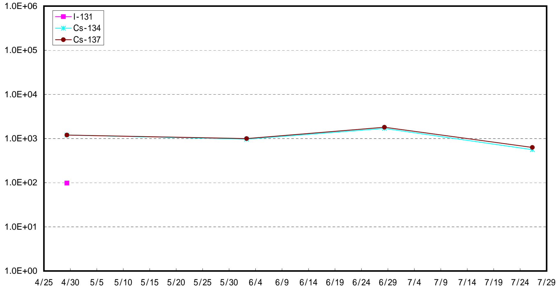
Radioactivity Density of Ocean Soil at 3km offshore of Iwasawa shore (Bq/kg)
