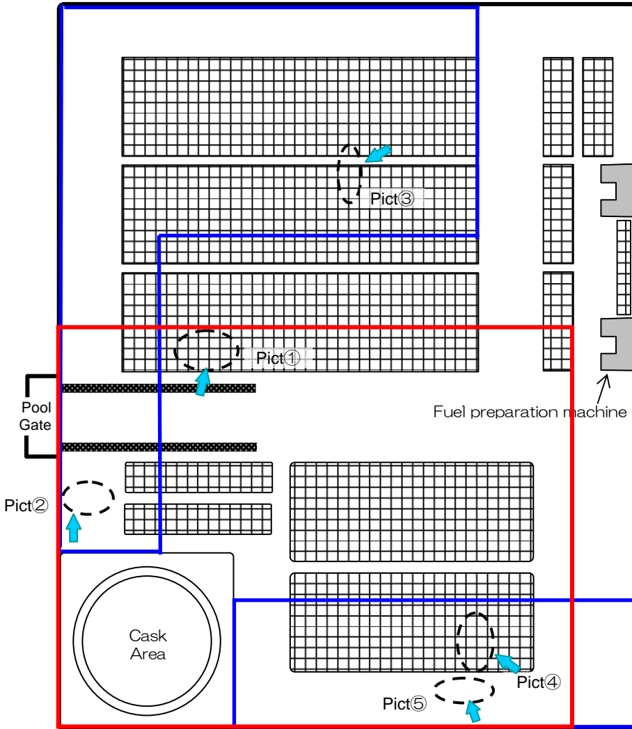
Pict① : Electric Motor of Fuel Exchanger
