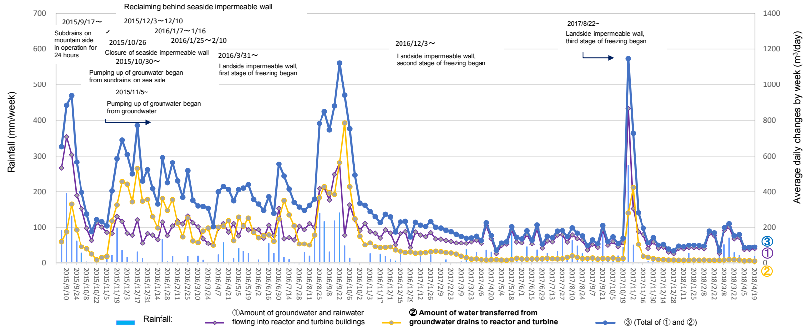
Amount of water transferred from groundwater drains to reactor and turbine buildings (From April 12, 2018 to April 18, 2018)
