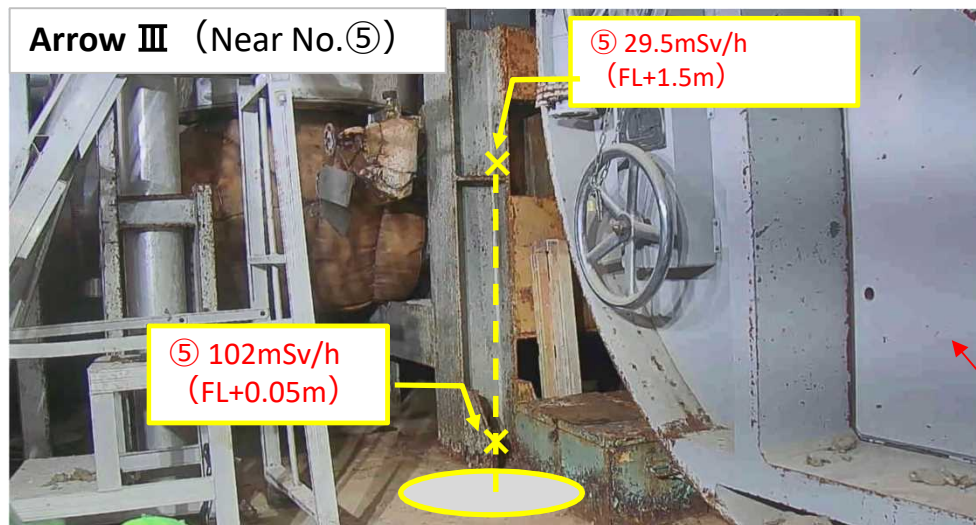
P/A room X-2 penetration
