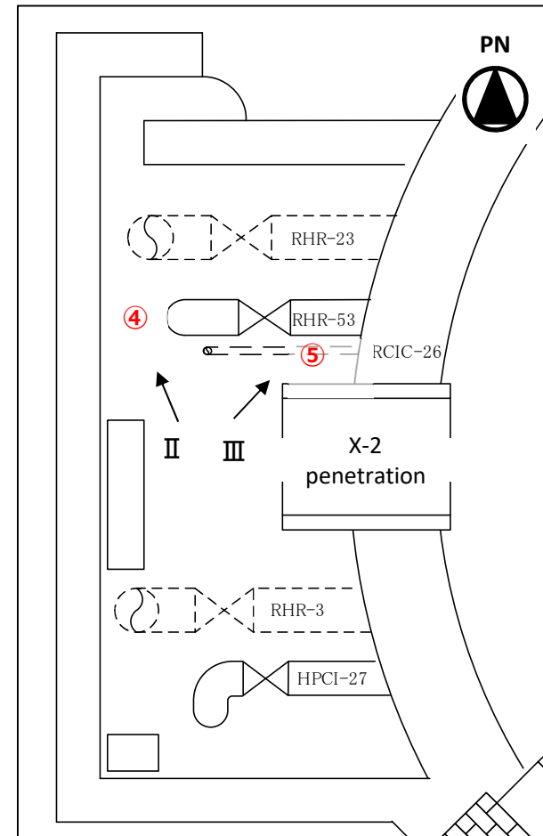
P/A room X-2 penetration
