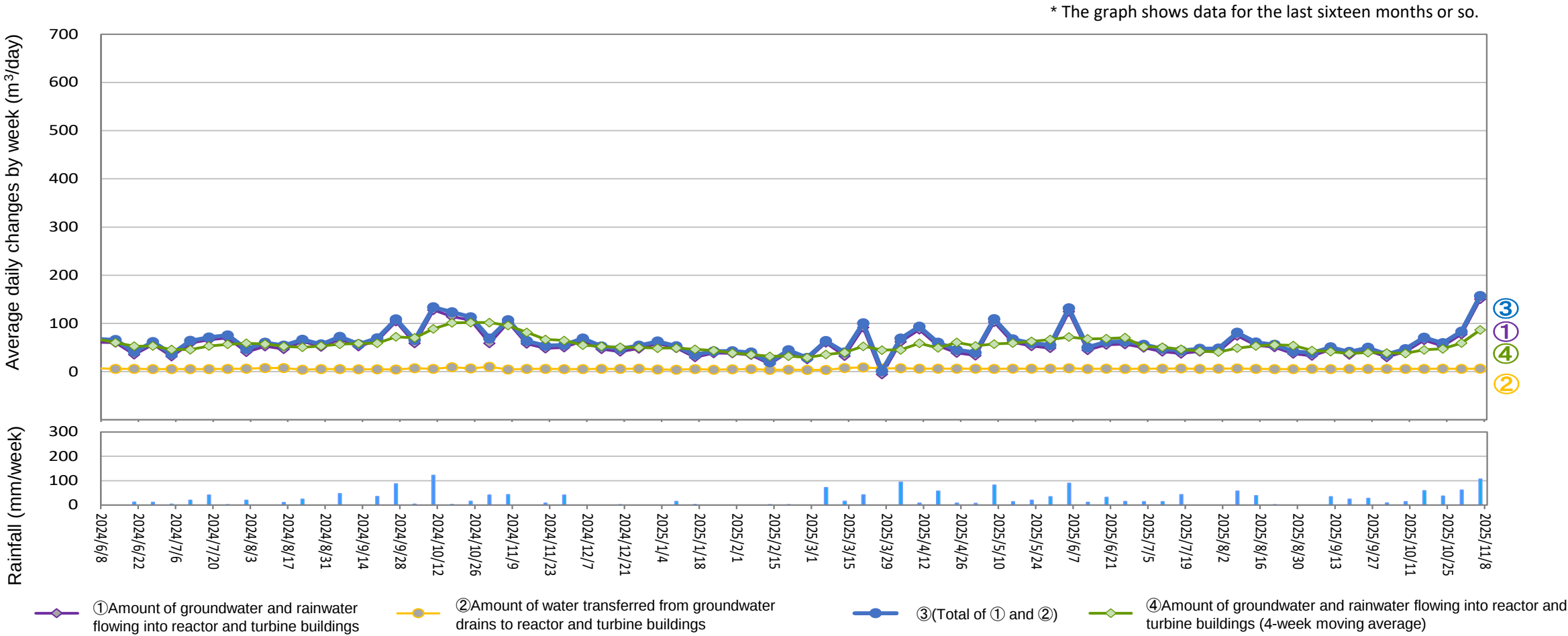
Amount of water transferred from groundwater drains to reactor and turbine buildings (From October 30, 2025 to November 5, 2025)
