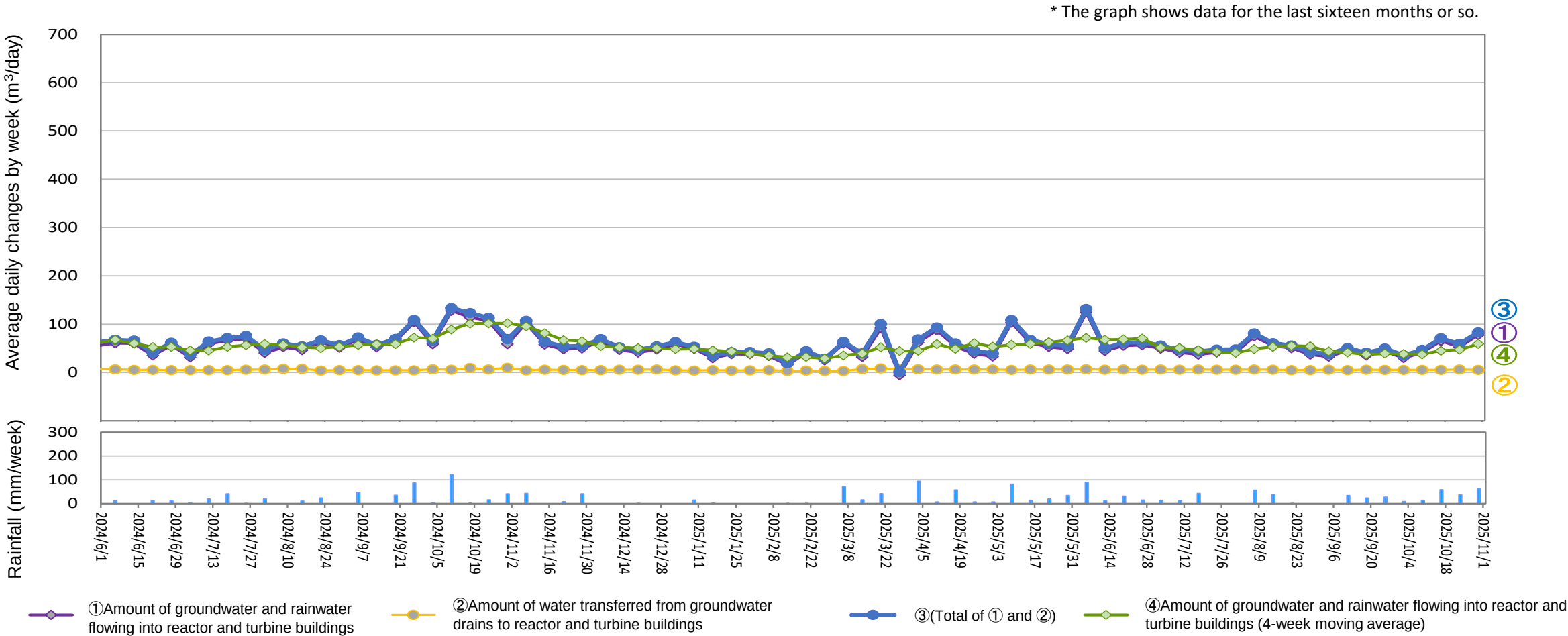
Amount of water transferred from groundwater drains to reactor and turbine buildings (From October 23, 2025 to October 29, 2025)
