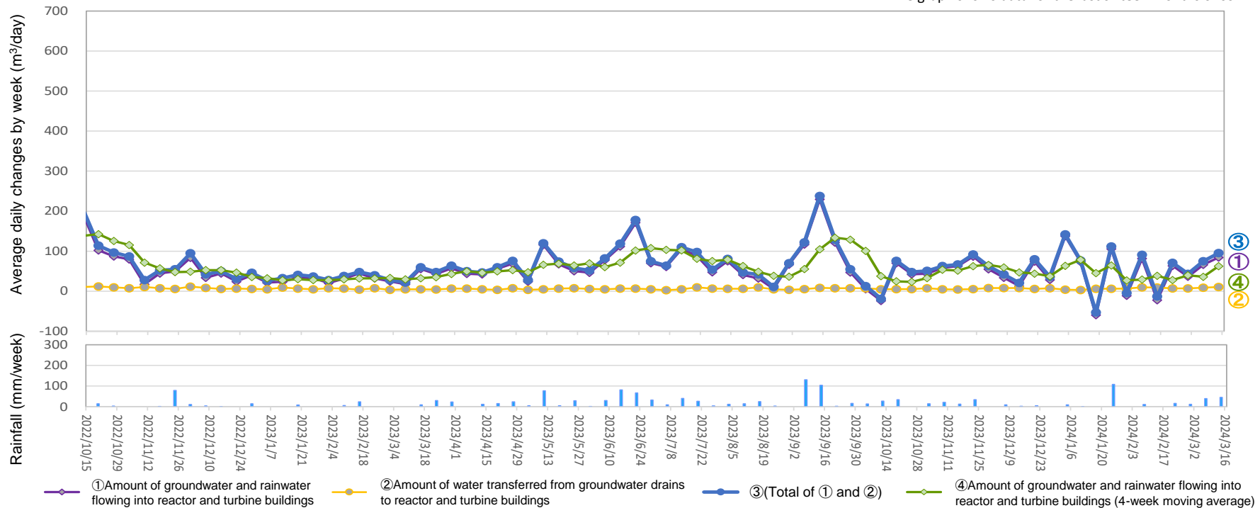
Amount of water transferred from groundwater drains to reactor and turbine buildings (From March 7, 2024 to March 13, 2024)
