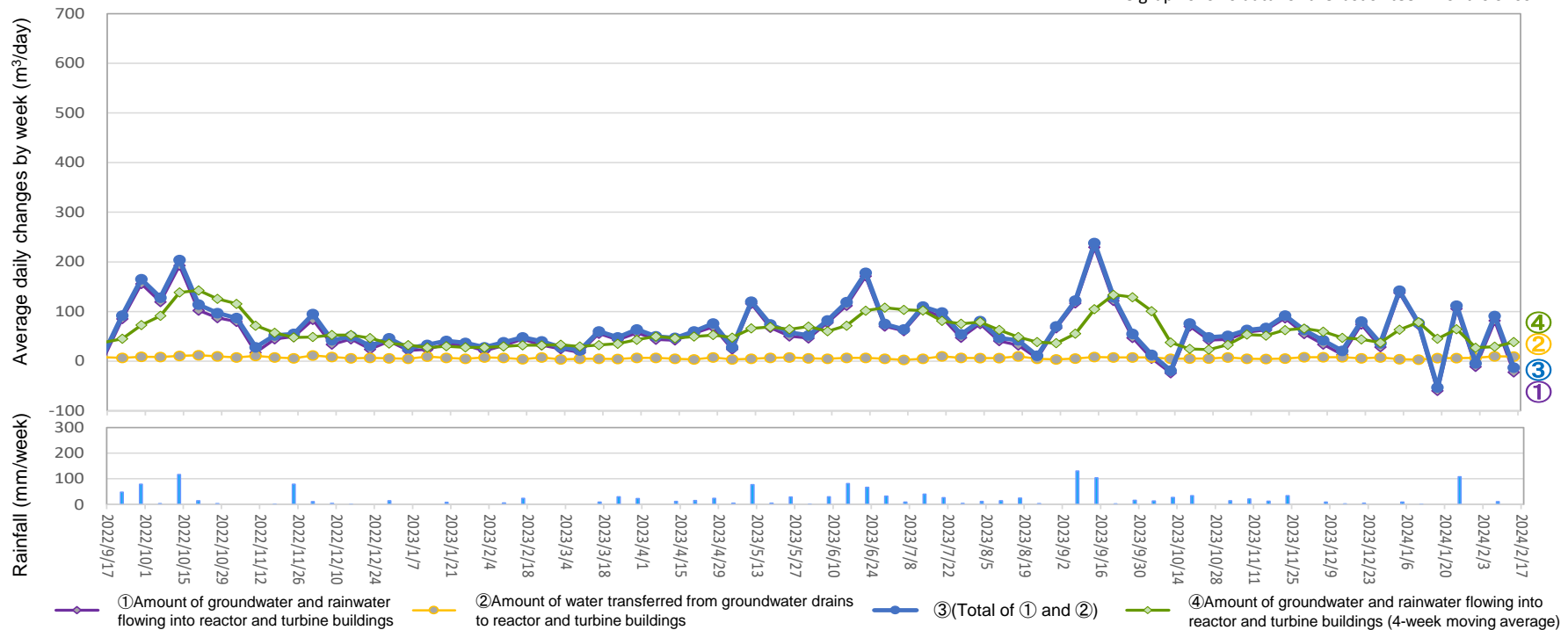
Amount of water transferred from groundwater drains to reactor and turbine buildings (From February 8, 2024 to February 14, 2024)
