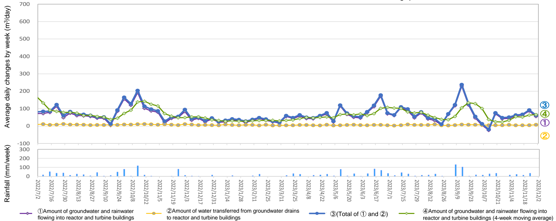
Amount of water transferred from groundwater drains to reactor and turbine buildings (From November 23, 2023 to November 29, 2023)
