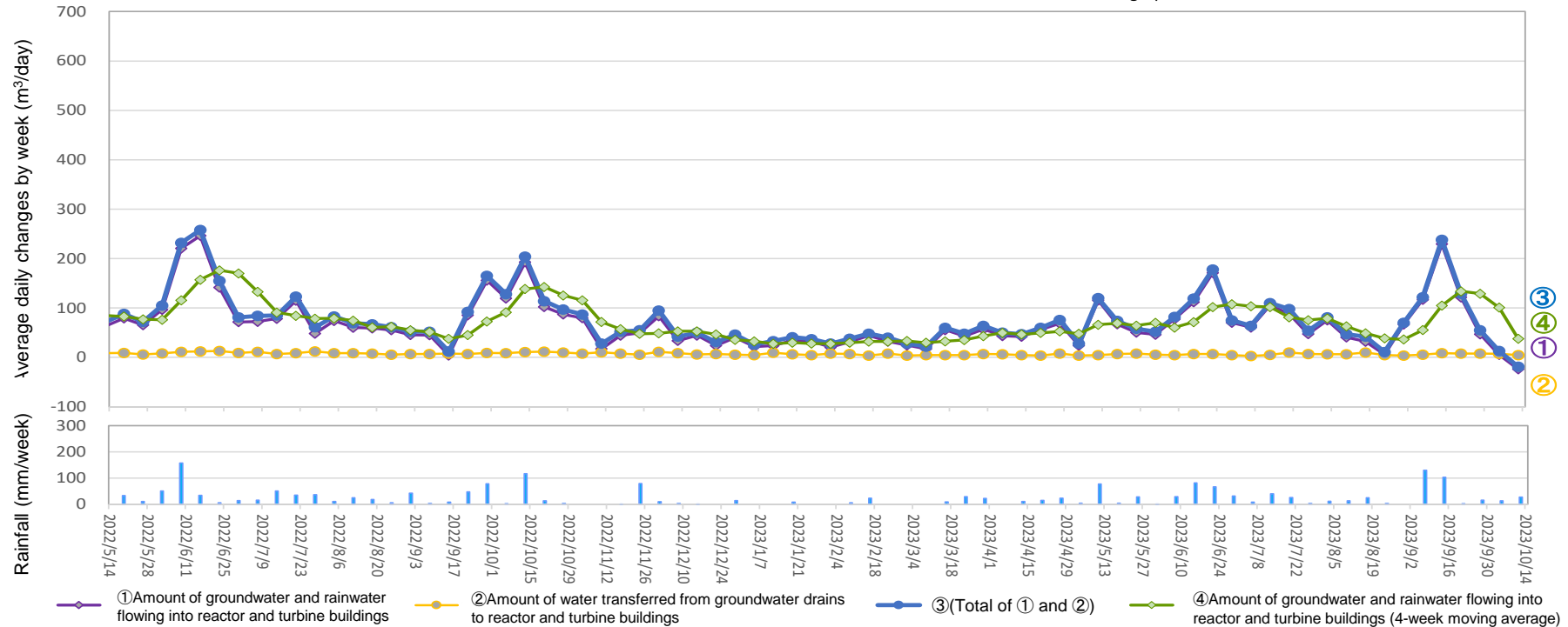
Amount of water transferred from groundwater drains to reactor and turbine buildings (From October 5, 2023 to October 11, 2023)
