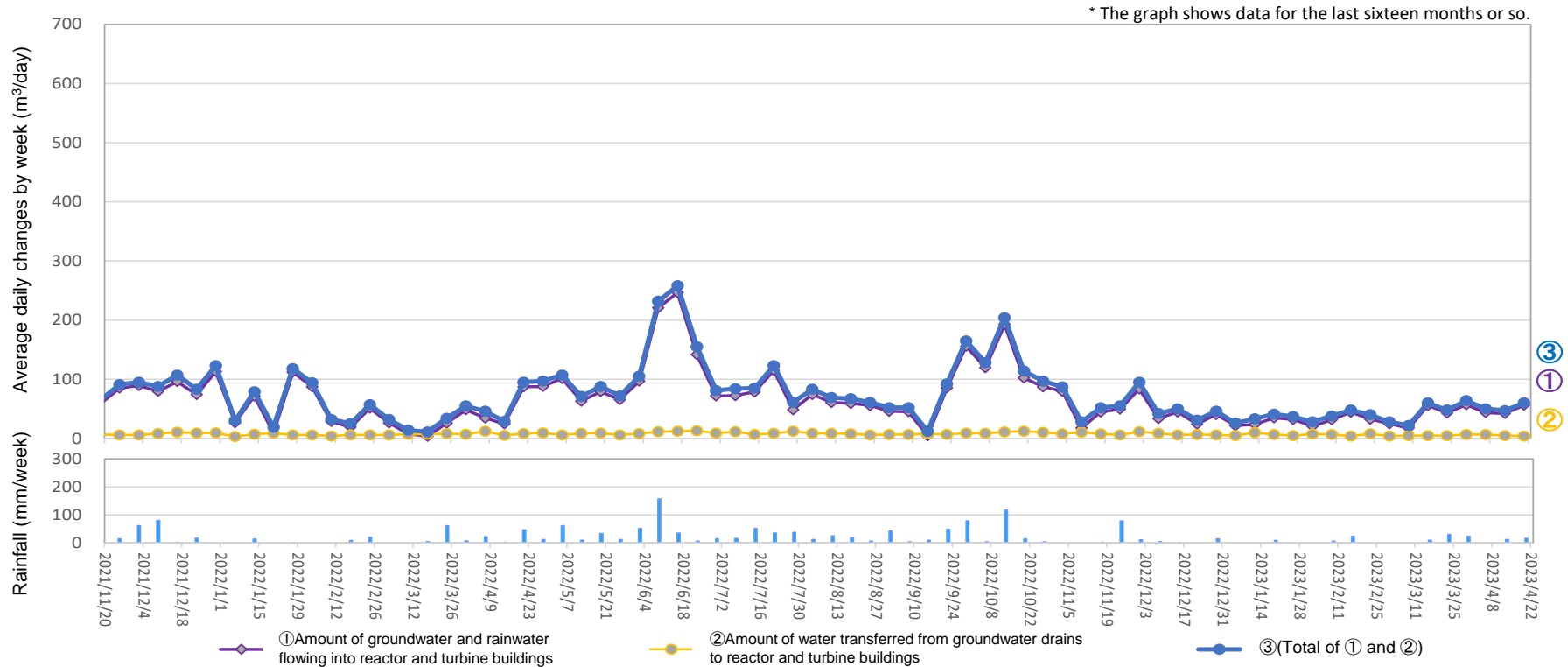
Amount of water transferred from groundwater drains to reactor and turbine buildings (From April 13, 2023 to April 19, 2023)
