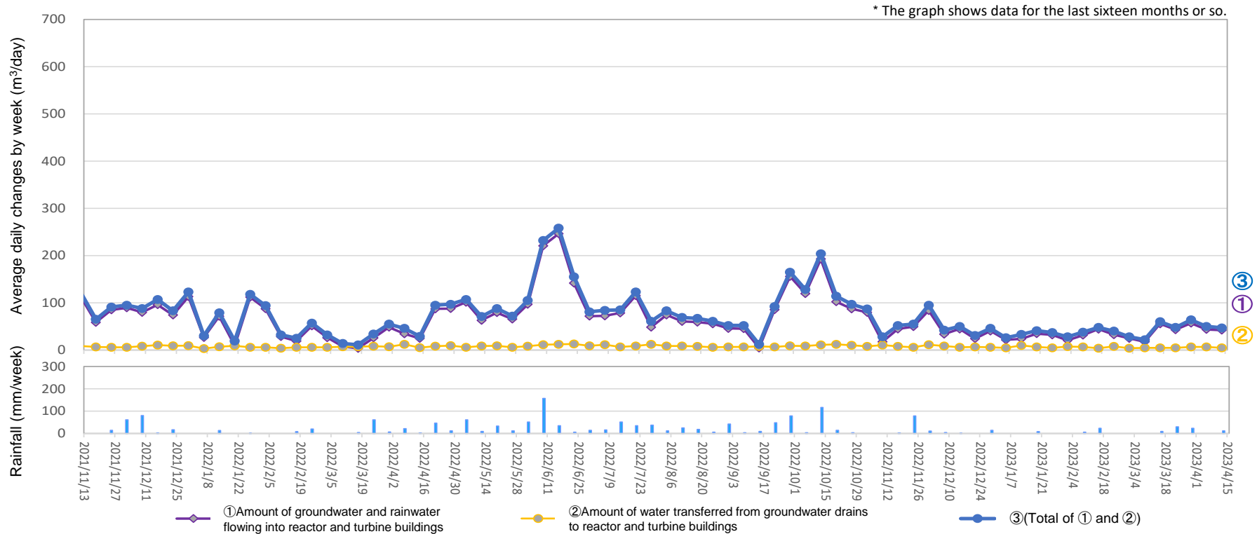
Amount of water transferred from groundwater drains to reactor and turbine buildings (From April 6, 2023 to April 12, 2023)
