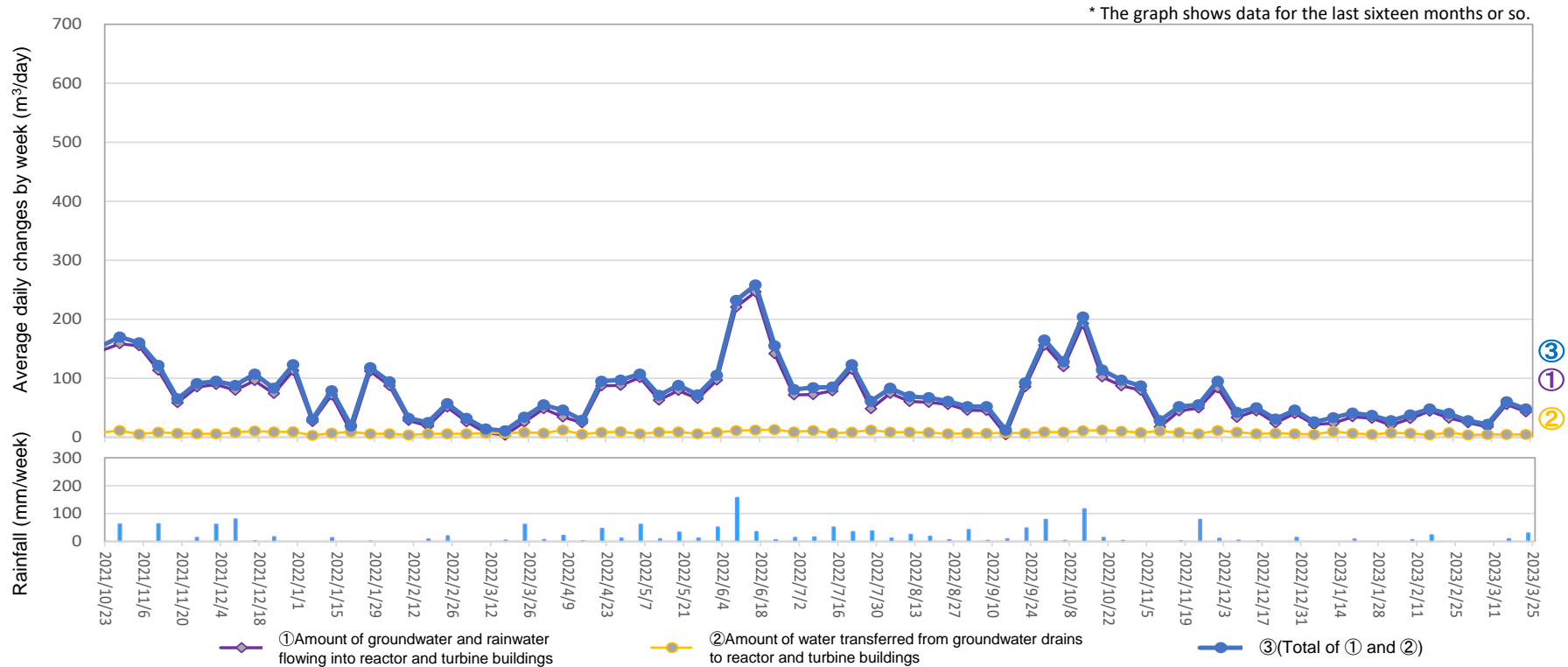
Amount of water transferred from groundwater drains to reactor and turbine buildings (From March 16, 2023 to March 22, 2023)
