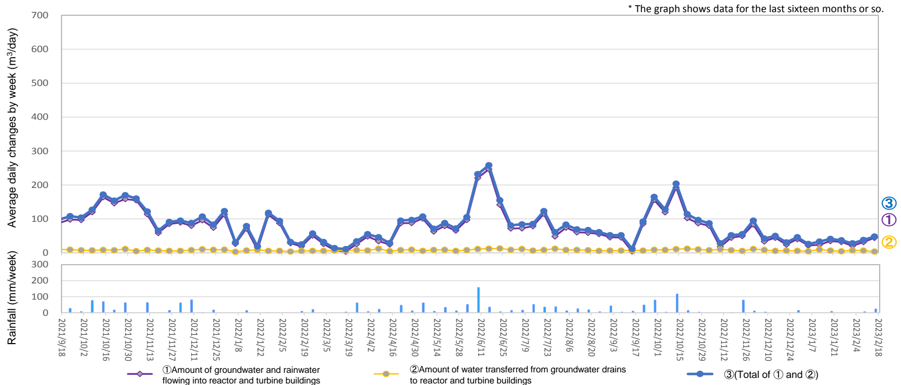
Amount of water transferred from groundwater drains to reactor and turbine buildings (From February 9, 2023 to February 15, 2023)
