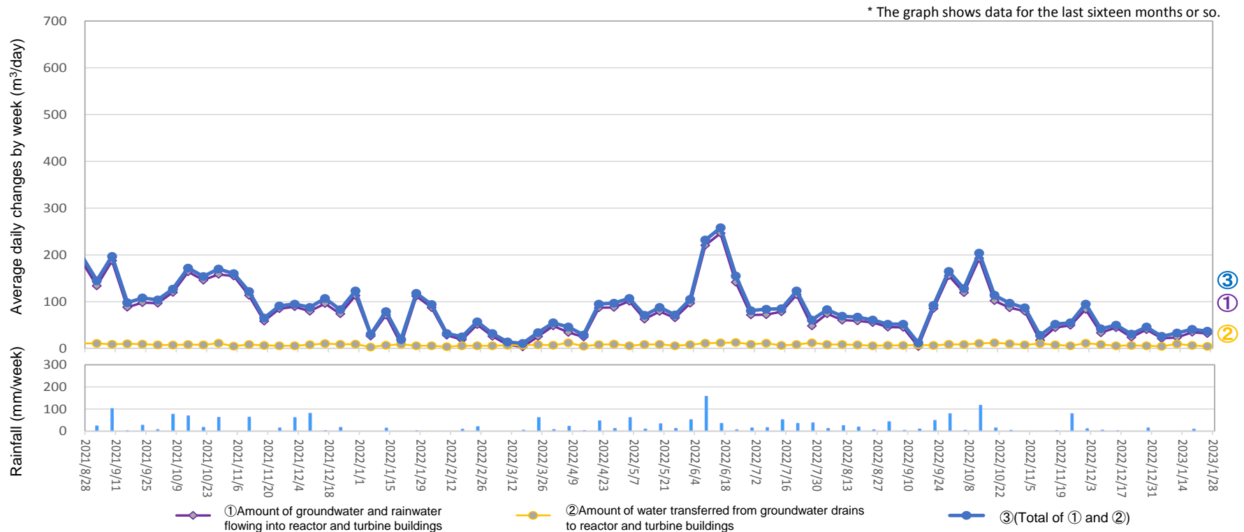
Amount of water transferred from groundwater drains to reactor and turbine buildings (From January 19, 2023 to January 25, 2023)
