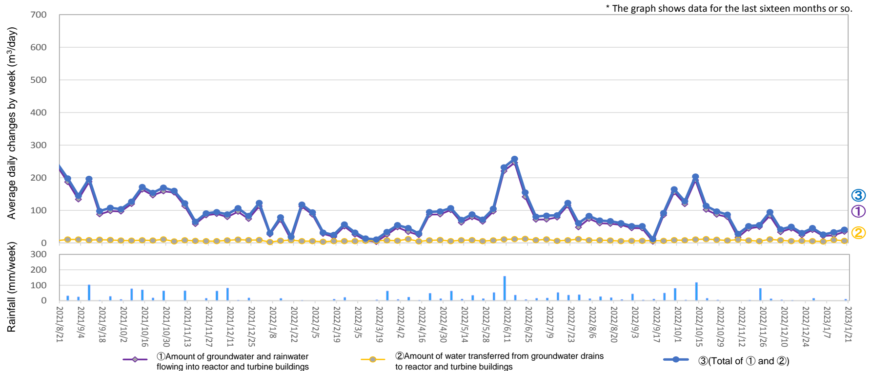
Amount of water transferred from groundwater drains to reactor and turbine buildings (From January 12, 2023 to January 18, 2023)
