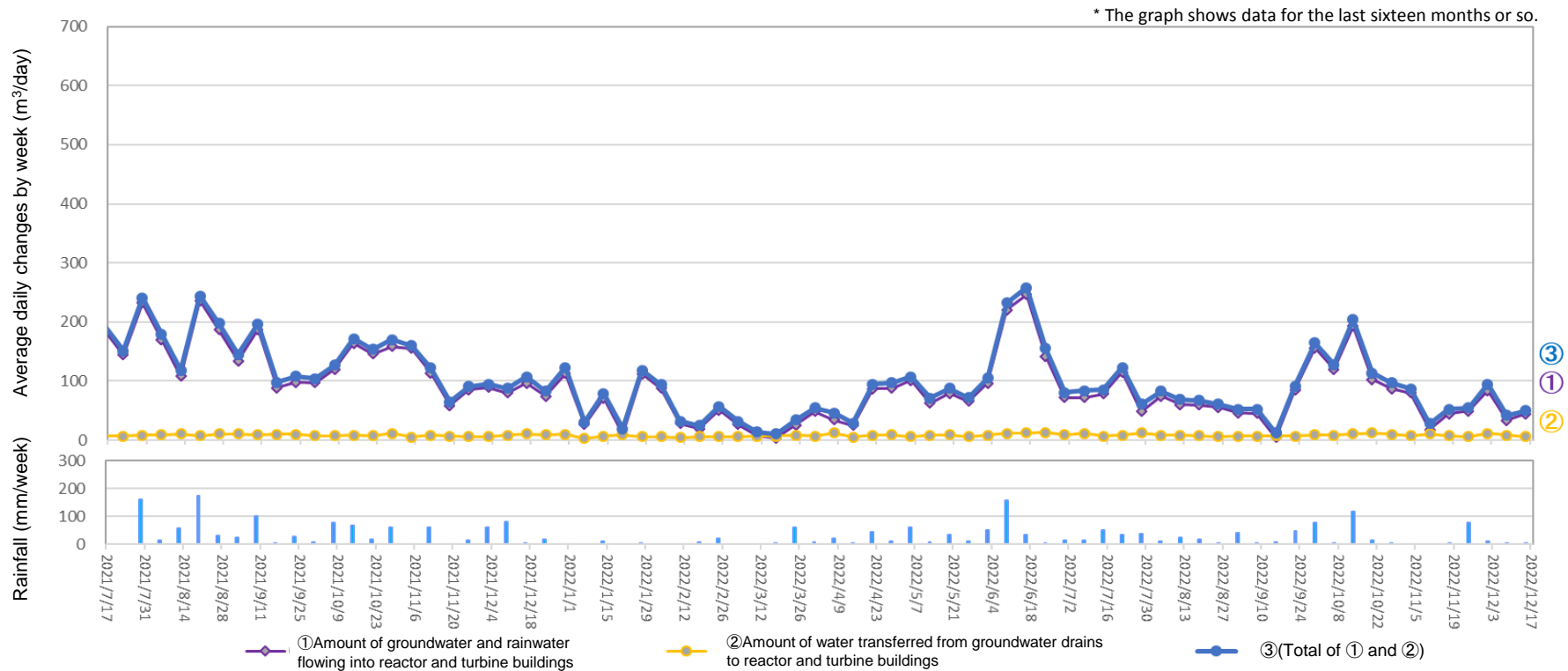
Amount of water transferred from groundwater drains to reactor and turbine buildings (From December 8, 2022 to December 14, 2022)
