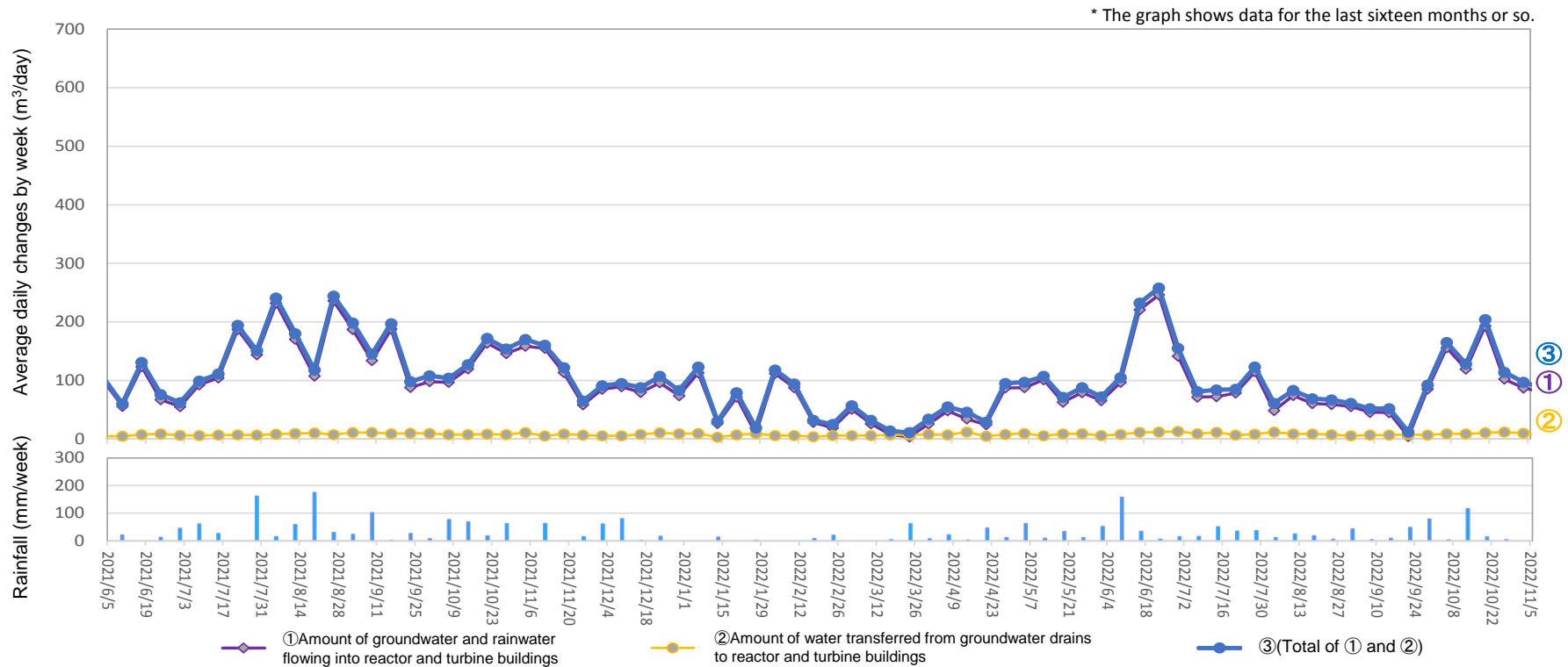
Amount of water transferred from groundwater drains to reactor and turbine buildings (From October 27, 2022 to November 2, 2022)
