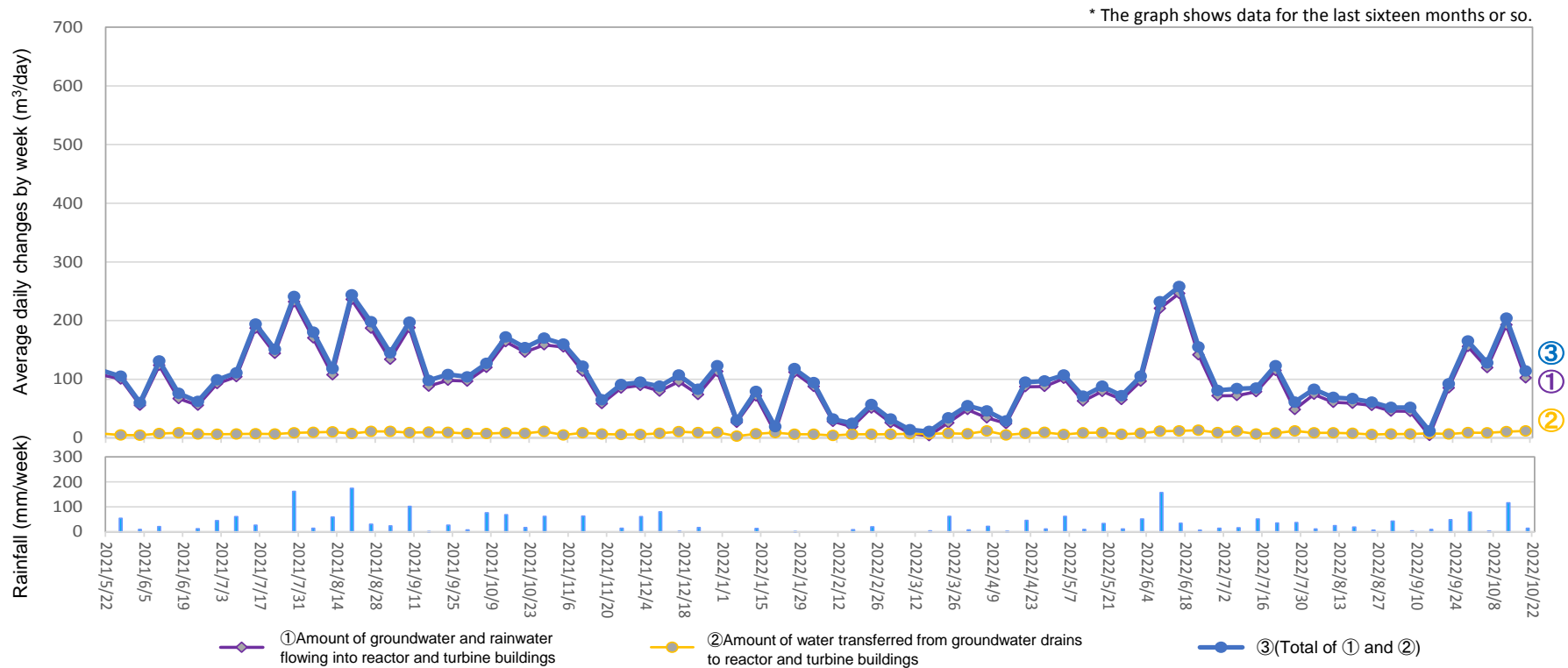
Amount of water transferred from groundwater drains to reactor and turbine buildings (From October 13, 2022 to October 19, 2022)
