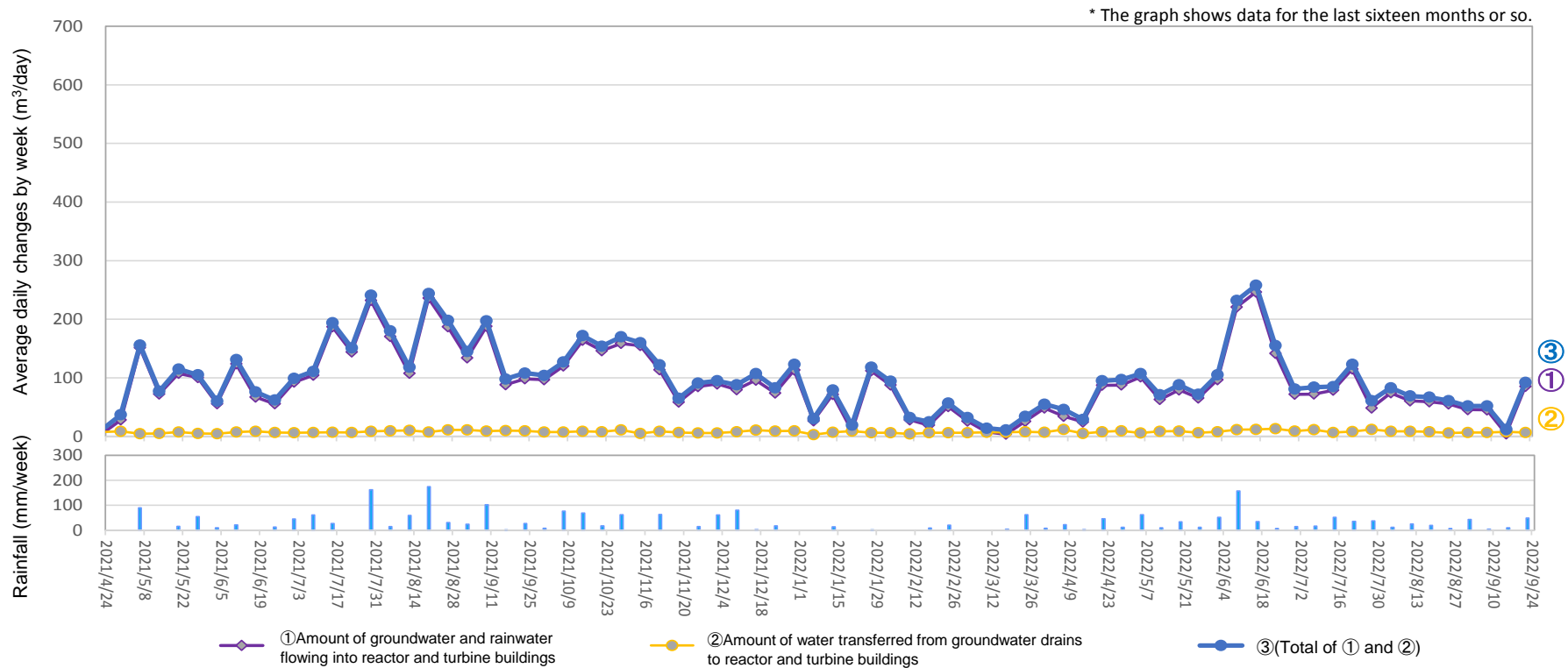
Amount of water transferred from groundwater drains to reactor and turbine buildings (From September 15, 2022 to September 21, 2022)
