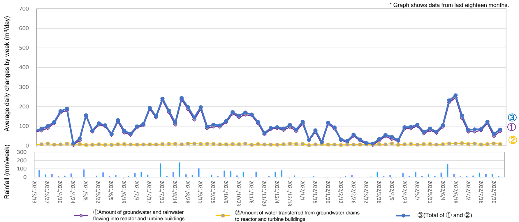
Amount of water transferred from groundwater drains to reactor and turbine buildings (From July 28, 2022 to August 3, 2022)
