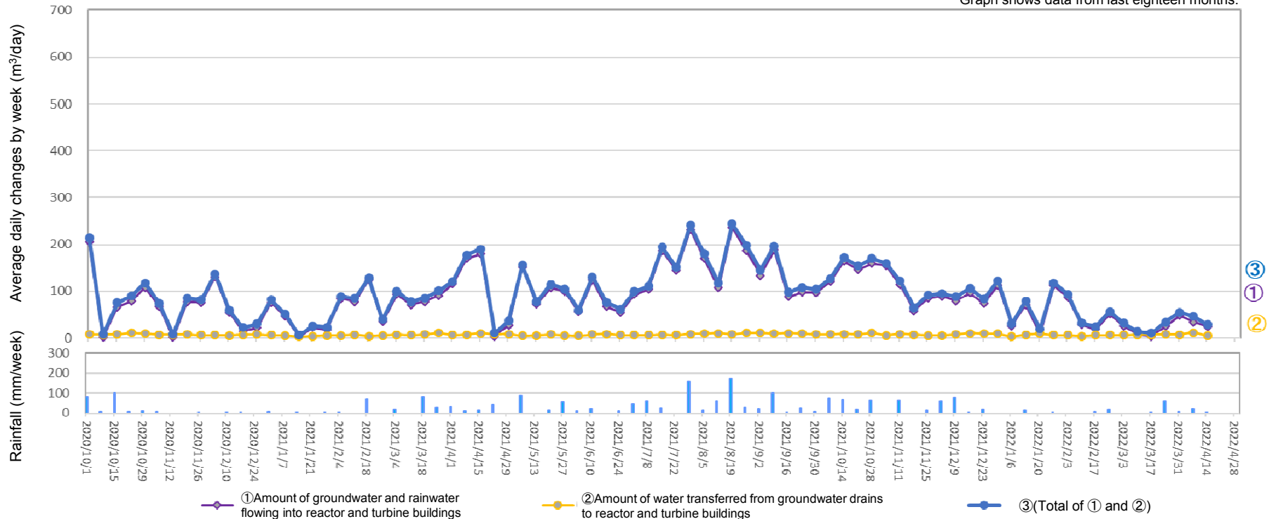
Amount of water transferred from groundwater drains to reactor and turbine buildings (From April 7, 2022 to April 13, 2022)
