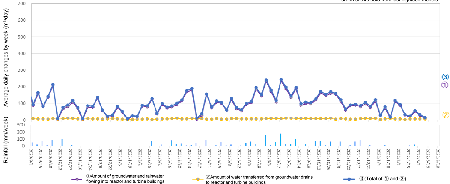
Amount of water transferred from groundwater drains to reactor and turbine buildings (From March 3, 2022 to March 9, 2022)
