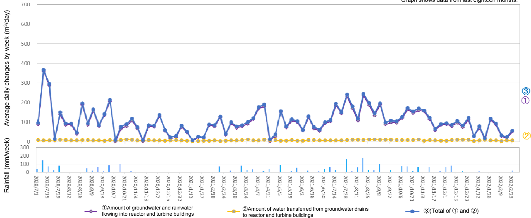
Amount of water transferred from groundwater drains to reactor and turbine buildings (From February 17, 2022 to February 23, 2022)
