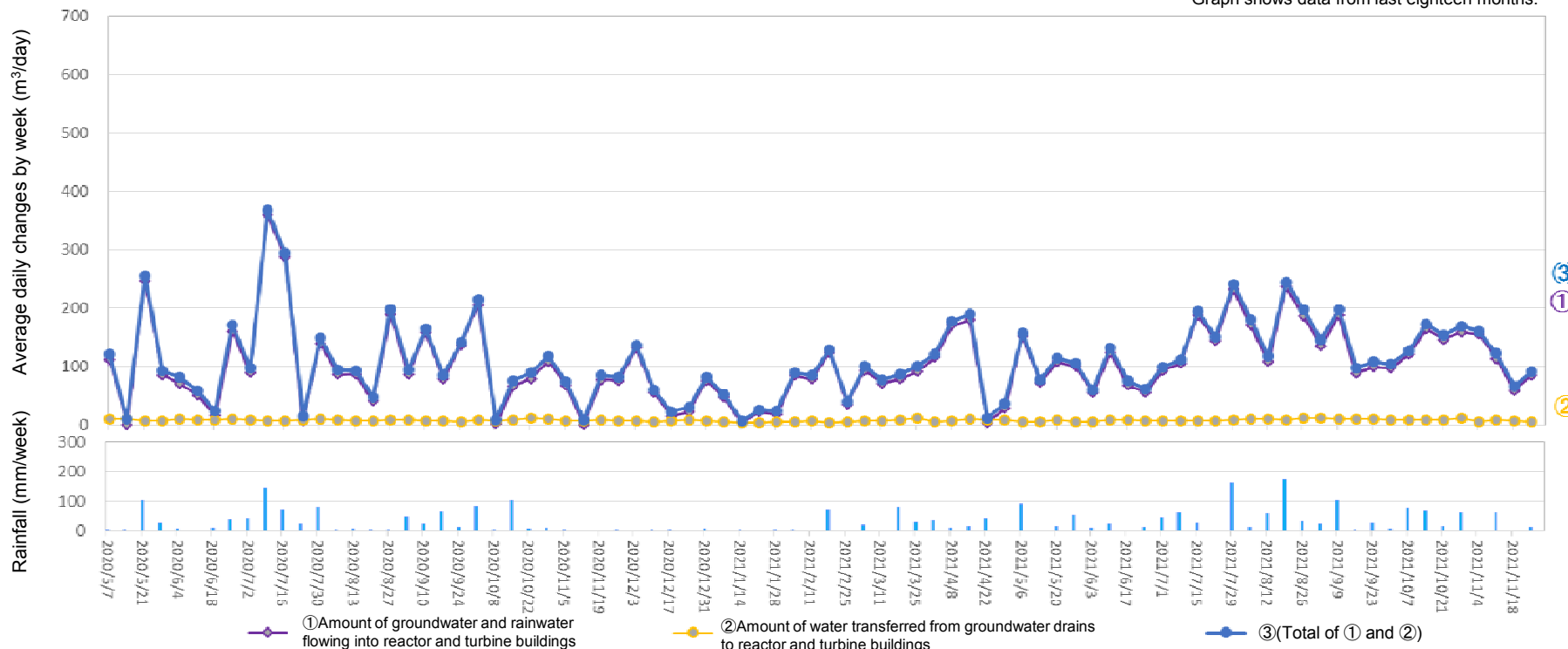
Amount of water transferred from groundwater drains to reactor and turbine buildings (From November 18, 2021 to November 24, 2021)
