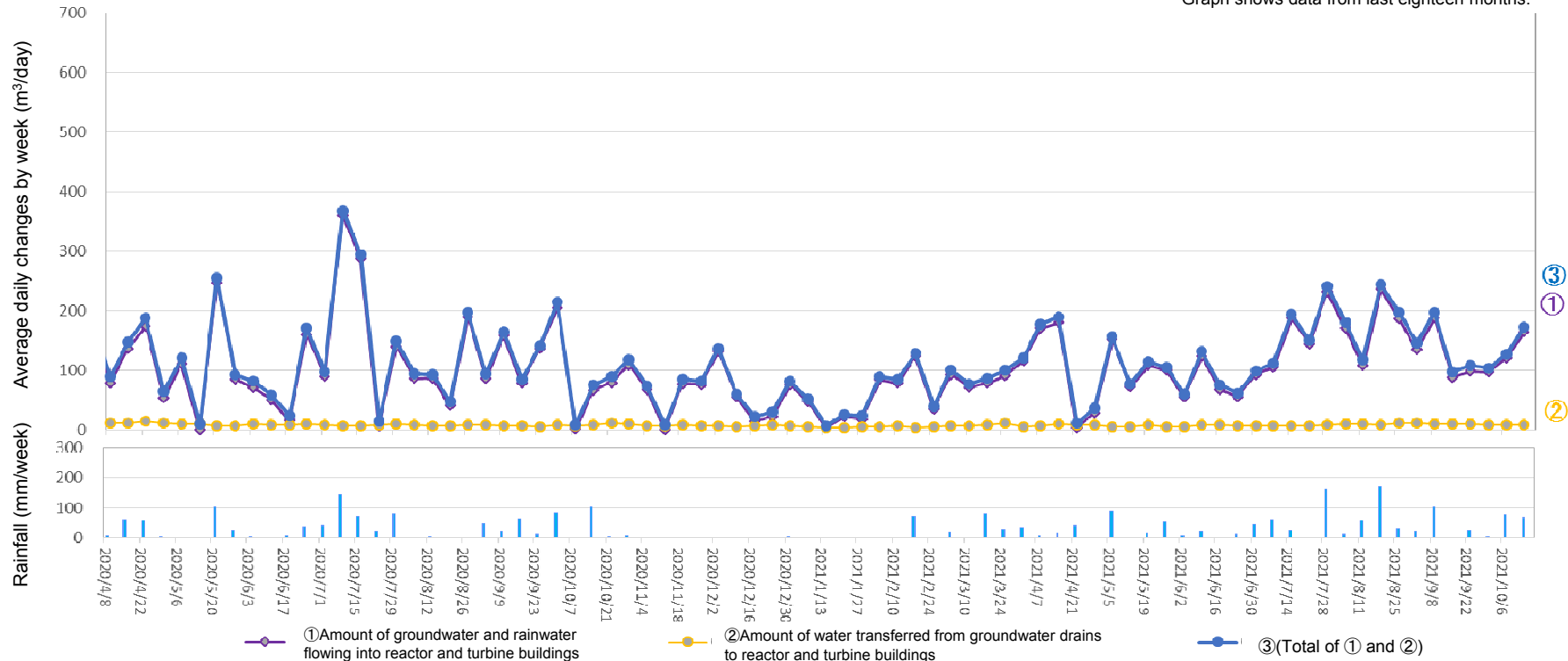
Amount of water transferred from groundwater drains to reactor and turbine buildings (From October 7, 2021 to October 13, 2021)
