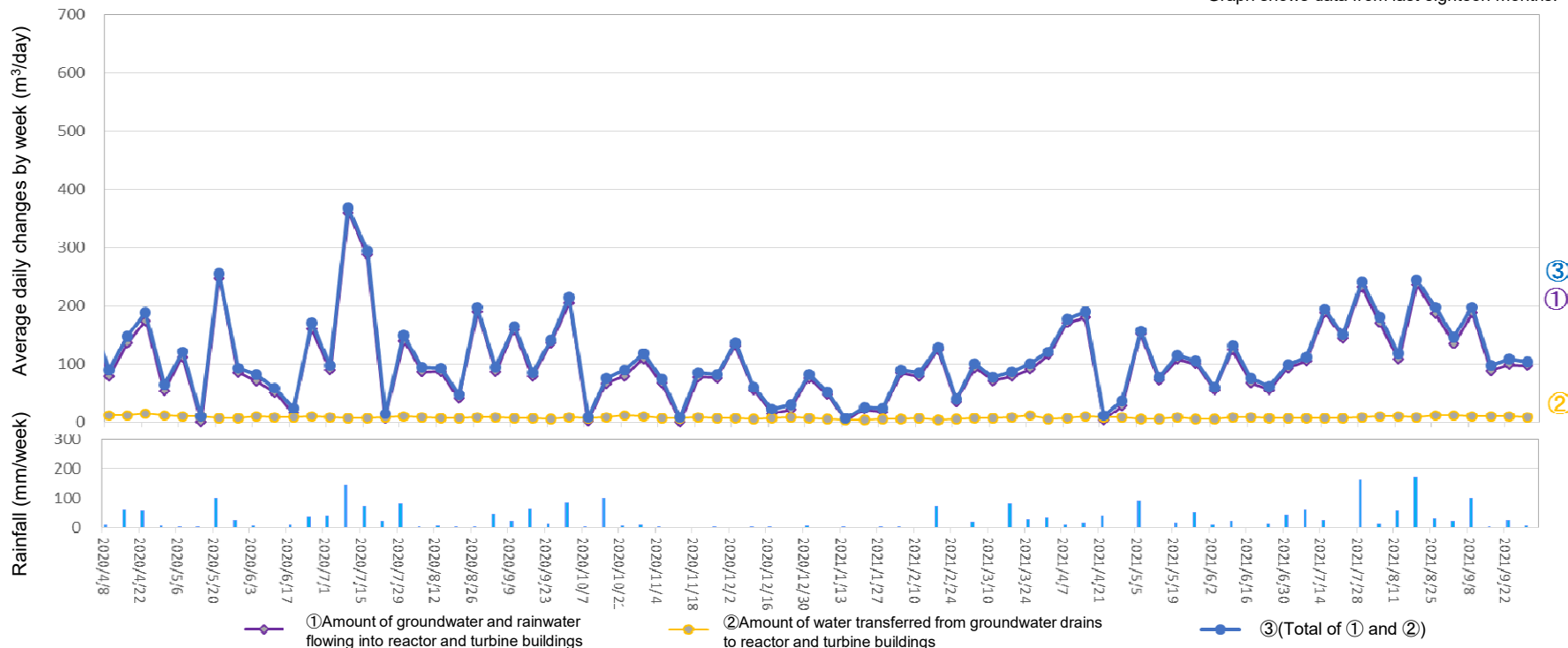
Amount of water transferred from groundwater drains to reactor and turbine buildings (From September 23, 2021 to September 29, 2021)
