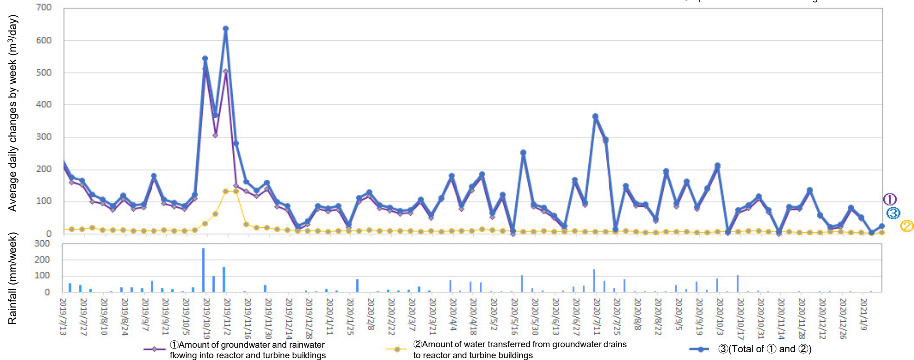
Amount of water transferred from groundwater drains to reactor and turbine buildings (From Jan 14, 2021 to Jan 20, 2021)
