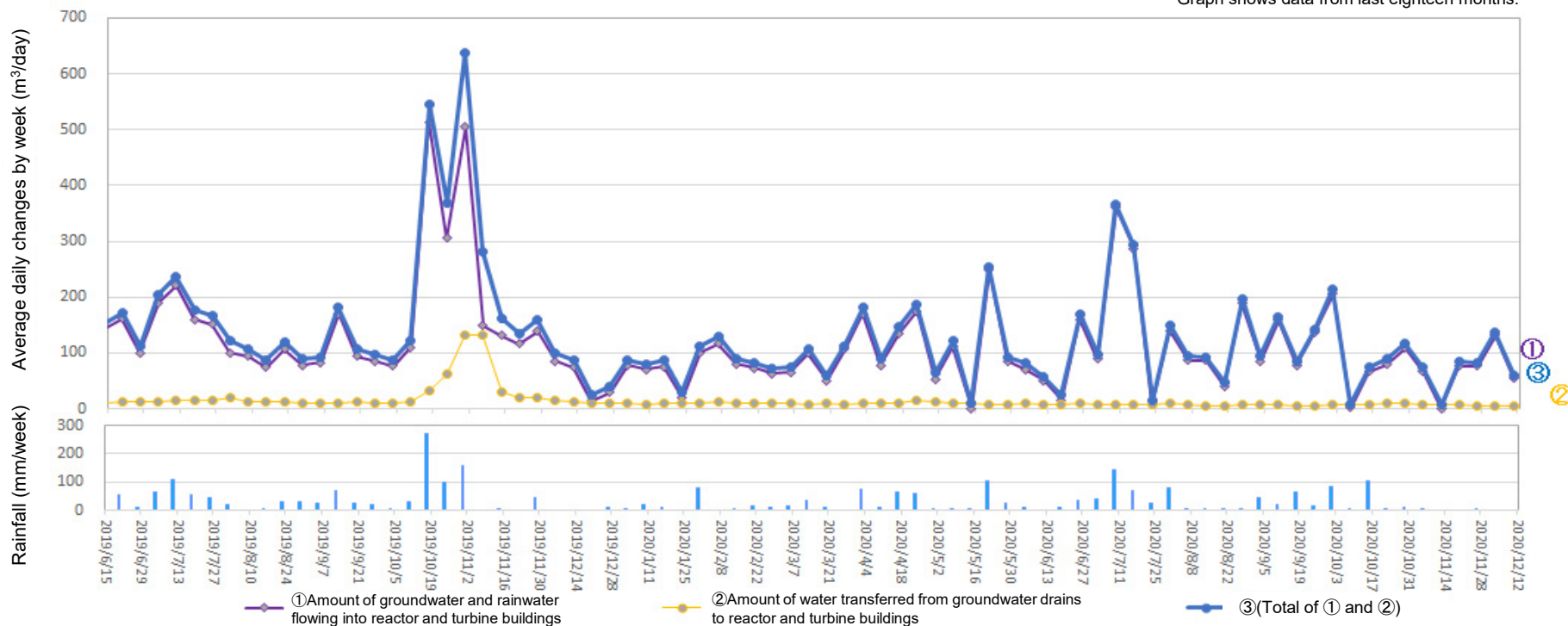
Amount of water transferred from groundwater drains to reactor and turbine buildings (From Dec 3, 2020 to Dec 9, 2020)
