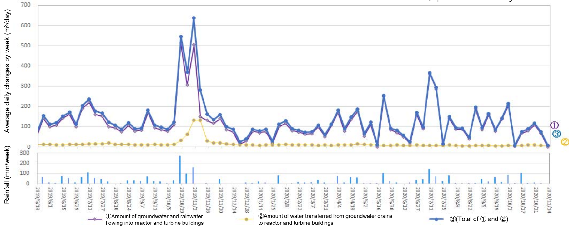
Amount of water transferred from groundwater drains to reactor and turbine buildings (From Nov 5, 2020 to Nov 11, 2020)
