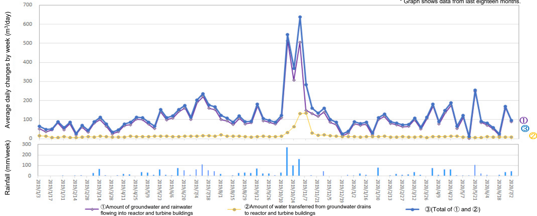
Amount of water transferred from groundwater drains to reactor and turbine buildings (From Jun 25, 2020 to Jul 1, 2020)
